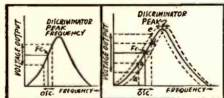
Figs. 2 and 3—How modulation takes place.
