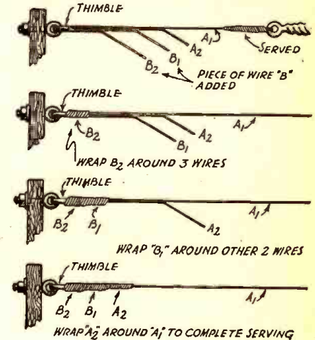
Fig. 3—Lead-ins for "T" and "inverted-L"
