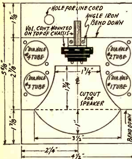
Chassis layout of the compact signal tracer.
