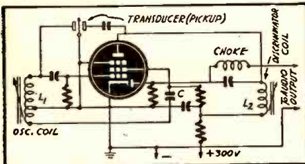
Fig. 4—A simple one-tube pickup circuit.
