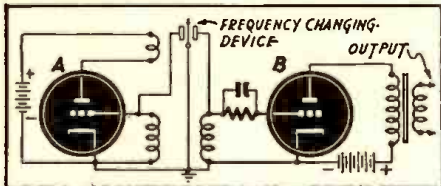
Fig. 1—Basic circuit of the new FM pickup.
