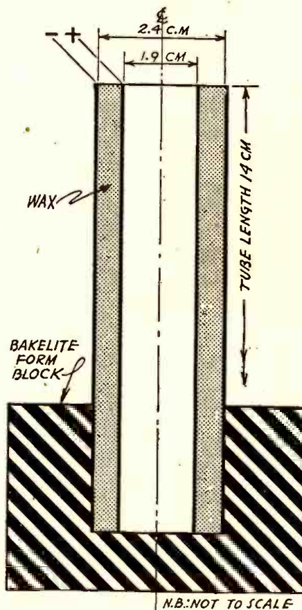
Fig. 1—Simple setup for making an electret.
