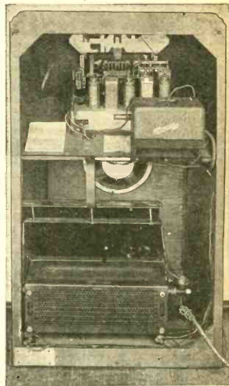
Back view of the gas-operated radio receiver.
